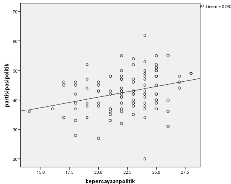
Gambar 1. Plot Hasil Uji Linearitas
